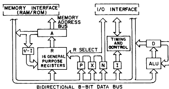
Fig. 1 — Microcomputer architecture.
